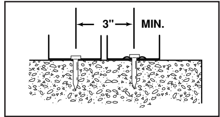
SPACING - THIN GAUGE METAL TO CONCRETE
